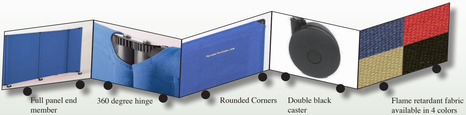
Mobile Partition 10' Long, 4', 6', or 6'10" High
